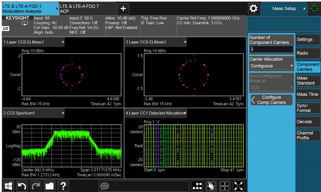
Figure 15. This display of an LTE downlink demodulation result includes the constellations of different signal layers (top) and detected resource allocations (bottom right).
