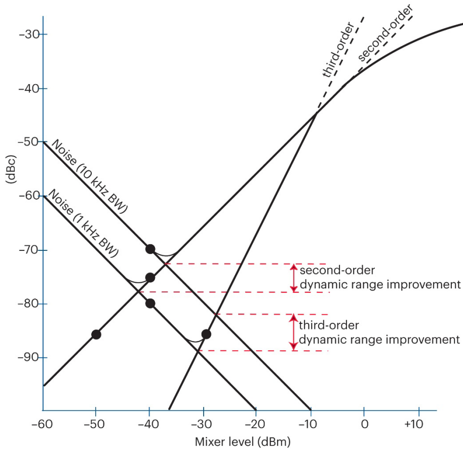
Figure 10. Reducing RBW lowers the analyzer's DANL (lines starting at lower left) and improves the operating point for both second- and third-order dynamic range.
