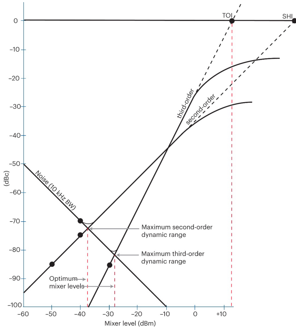
Figure 9. Second- and third-order dynamic range are shown as determined by minimum distortion regions at the intersection of DANL and the corresponding distortion curves.
