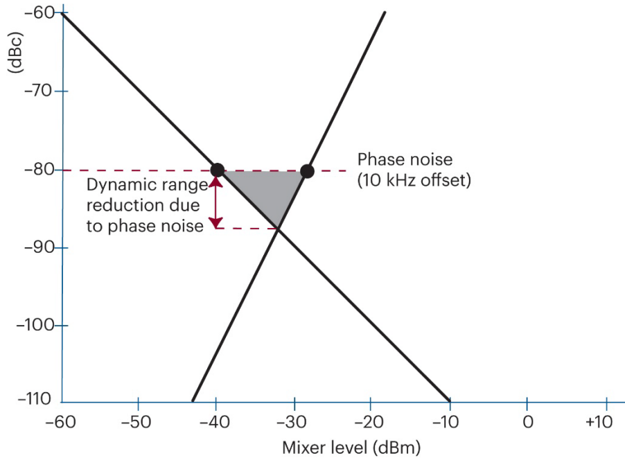
Figure 11. For closely spaced signals such as intermodulation test tones, phase noise may limit the measurement dynamic range to a value less than that the chart would suggest.
